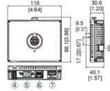
Rear Module (for all GP units)
