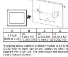
Panel Cut-out (for all GP units)
